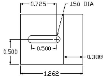
Part # CB975S
