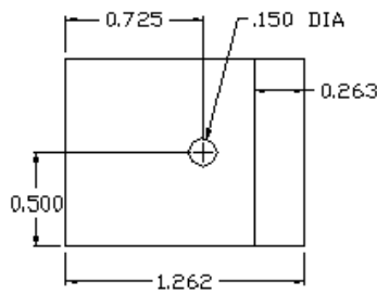
Part # CB970
