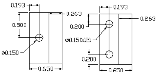
Part # CB962
