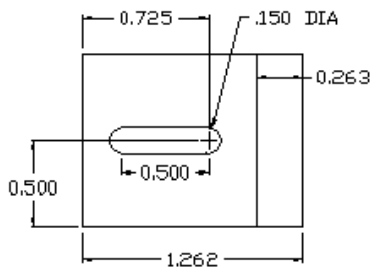
Part # CB970S
