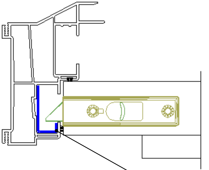
Jamb Reinforcement Clip
